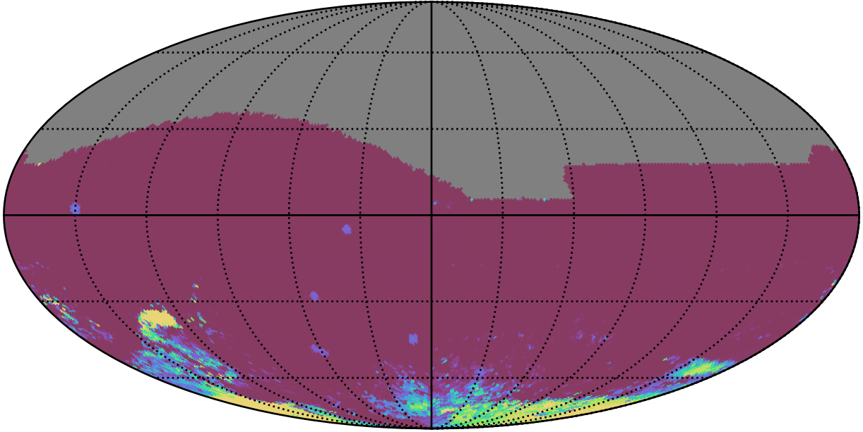
ddf_loaded_fl2_v3.4_10yrs All sky ri bands: 75th Percentile Intranight Timespan
