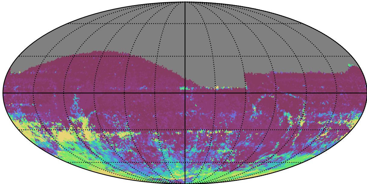
ddf_loaded_fl2_v3.4_10yrs All sky r band: 75th Percentile Intranight Timespan
