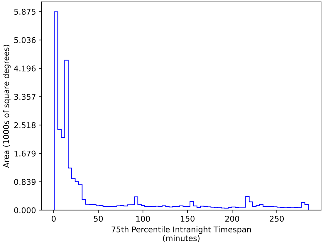
ddf_loaded_fl2_v3.4_10yrs All sky r band: 75th Percentile Intranight Timespan
