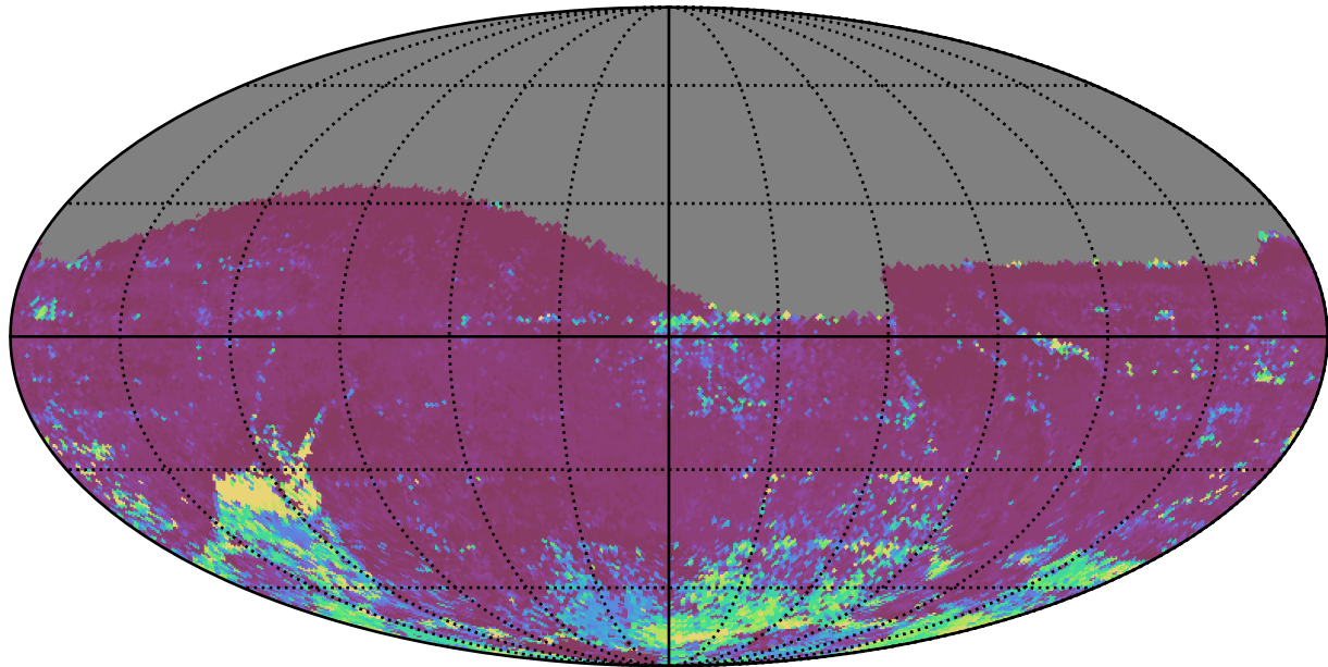
ddf_loaded_fl2_v3.4_10yrs All sky i band: 75th Percentile Intranight Timespan
