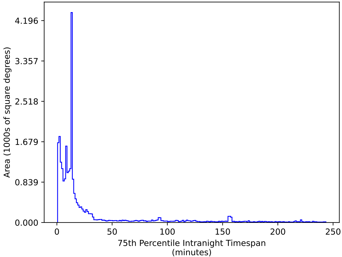
ddf_loaded_fl2_v3.4_10yrs All sky i band: 75th Percentile Intranight Timespan
