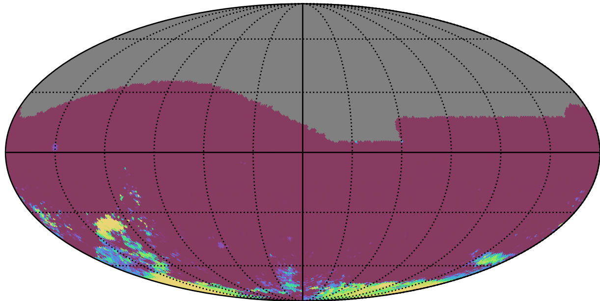
ddf_loaded_fl2_v3.4_10yrs All sky gr bands: 75th Percentile Intranight Timespan
