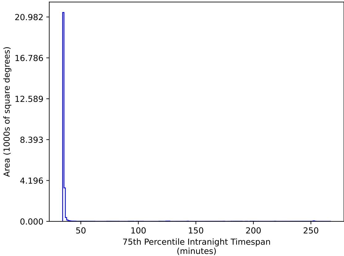
ddf_loaded_fl2_v3.4_10yrs All sky gr bands: 75th Percentile Intranight Timespan
