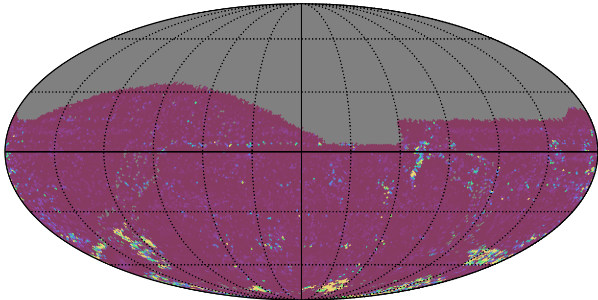
ddf_loaded_fl2_v3.4_10yrs All sky g band: 75th Percentile Intranight Timespan
