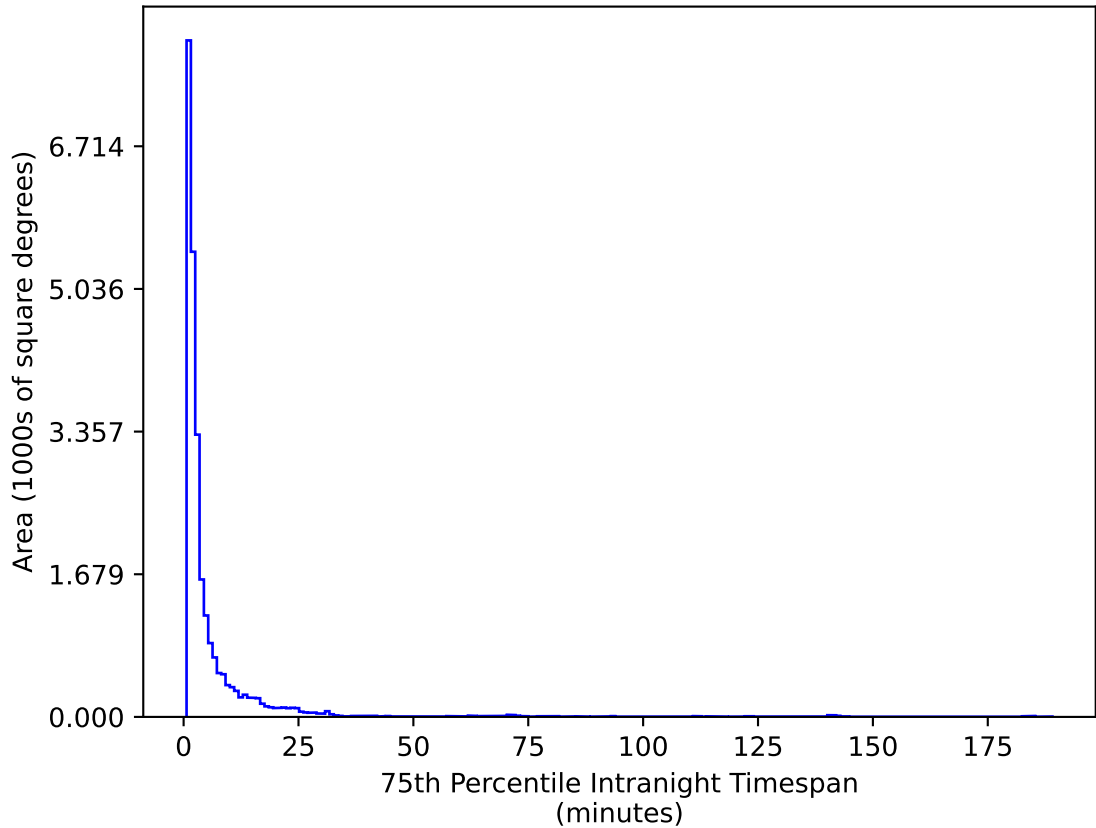
ddf_loaded_fl2_v3.4_10yrs All sky g band: 75th Percentile Intranight Timespan
