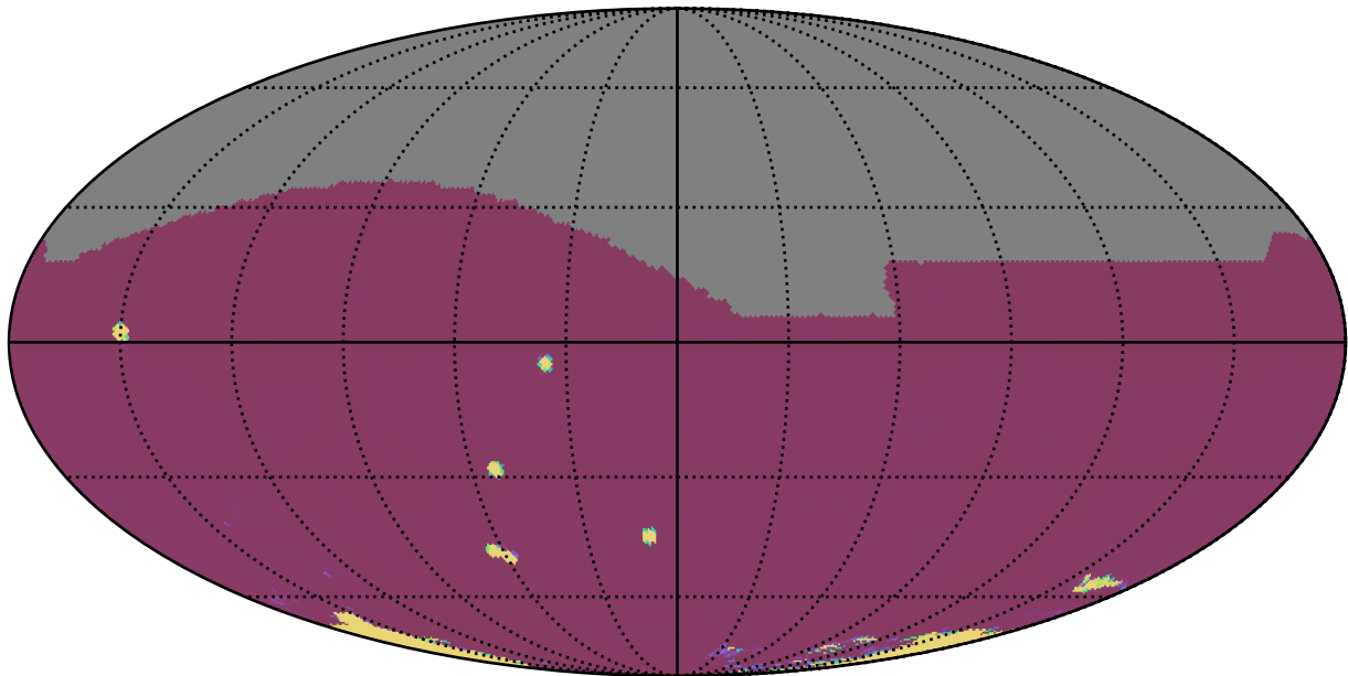
ddf_loaded_fl2_v3.4_10yrs All sky all bands: 75th Percentile Intranight Timespan
