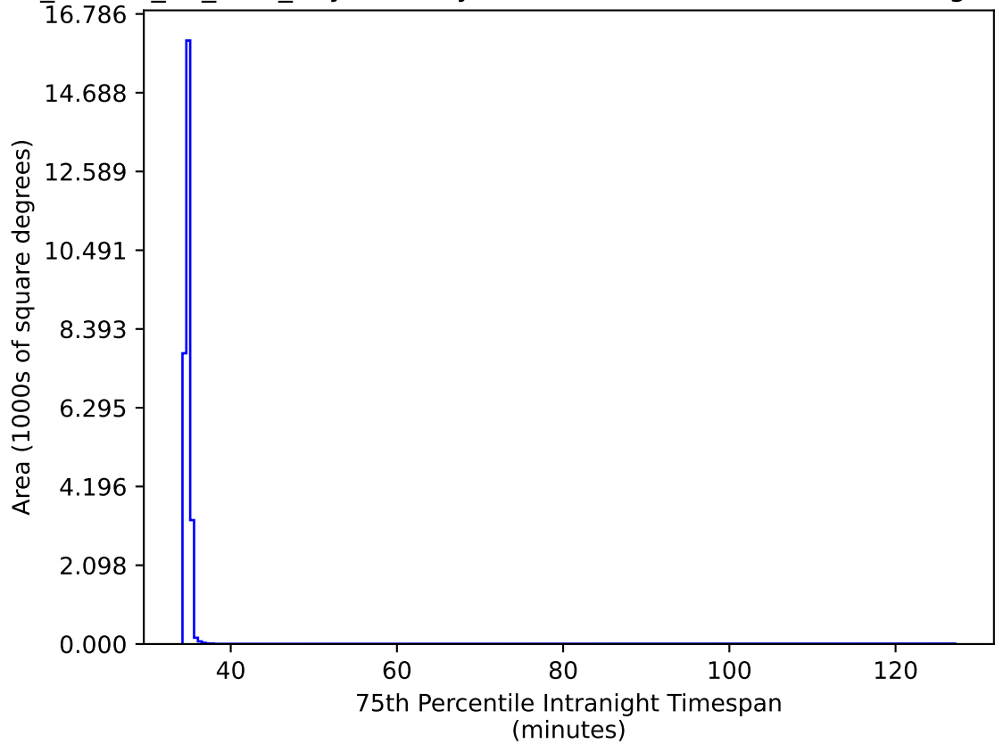
ddf_loaded_fl2_v3.4_10yrs All sky all bands: 75th Percentile Intranight Timespan
