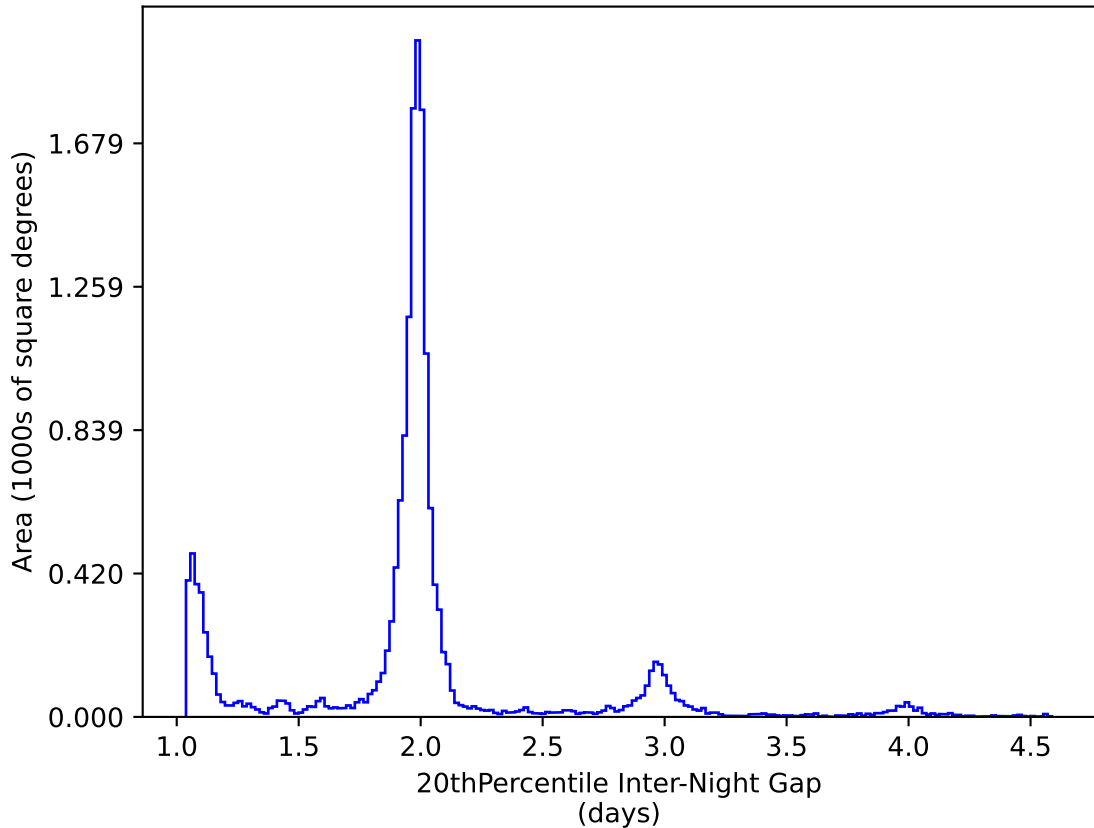
ddf_loaded_fl2_v3.4_10yrs WFD y band: 20thPercentile Inter-Night Gap
