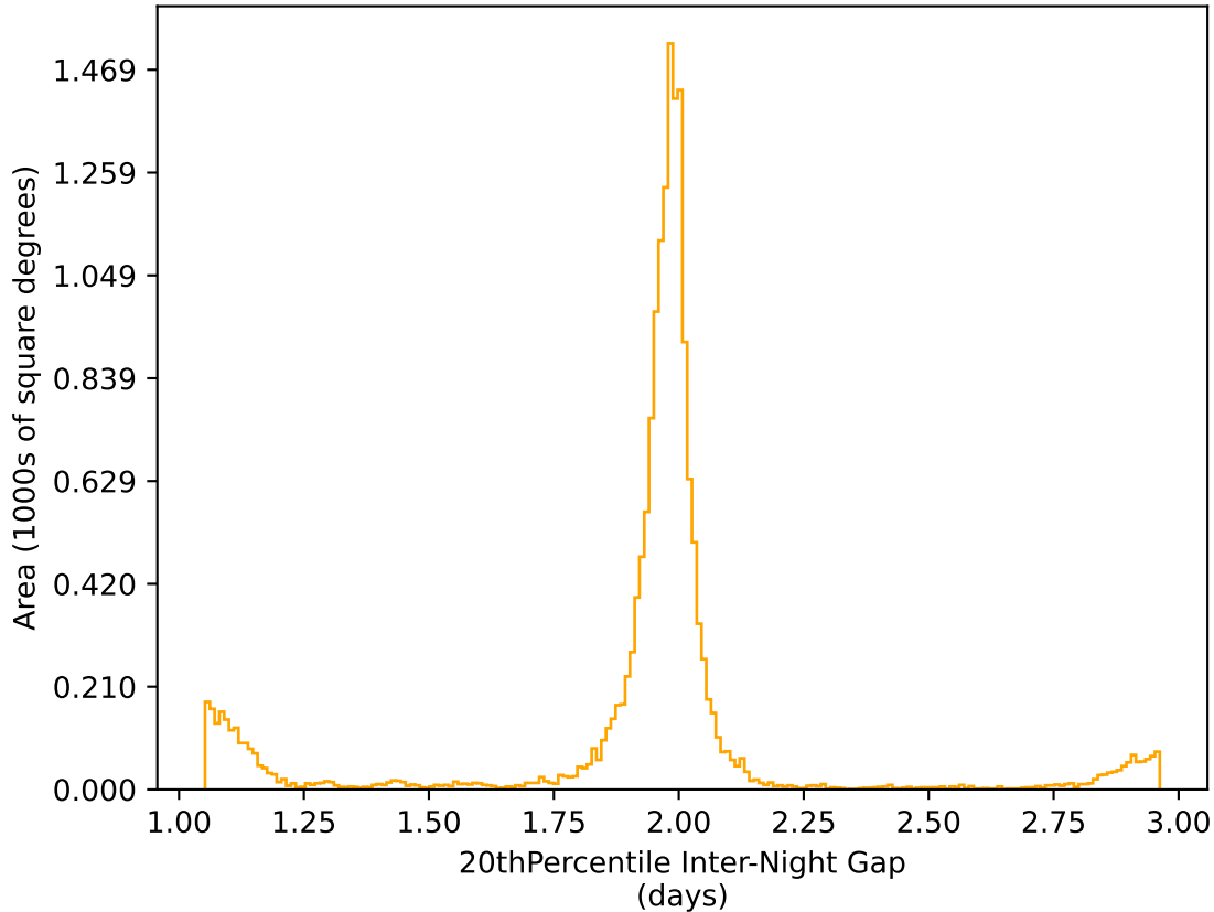
ddf_loaded_fl2_v3.4_10yrs WFD r band: 20thPercentile Inter-Night Gap
