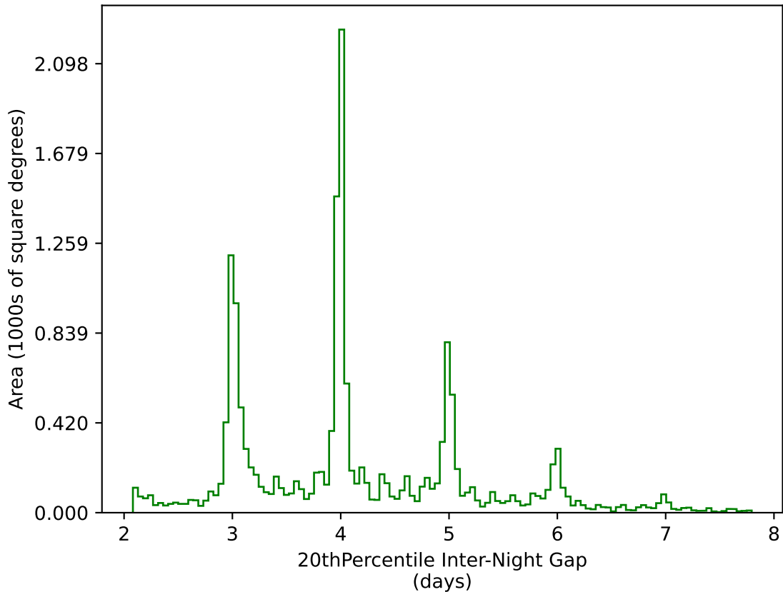
ddf_loaded_fl2_v3.4_10yrs WFD g band: 20thPercentile Inter-Night Gap
