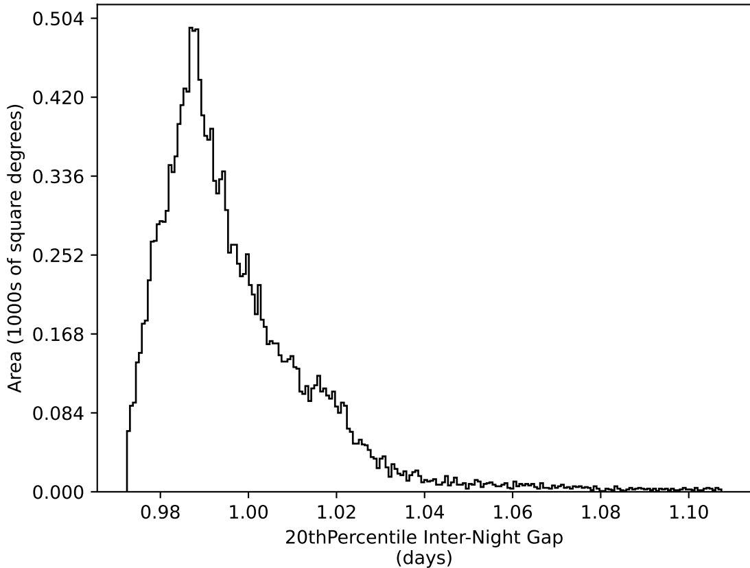
ddf_loaded_fl2_v3.4_10yrs WFD all bands: 20thPercentile Inter-Night Gap
