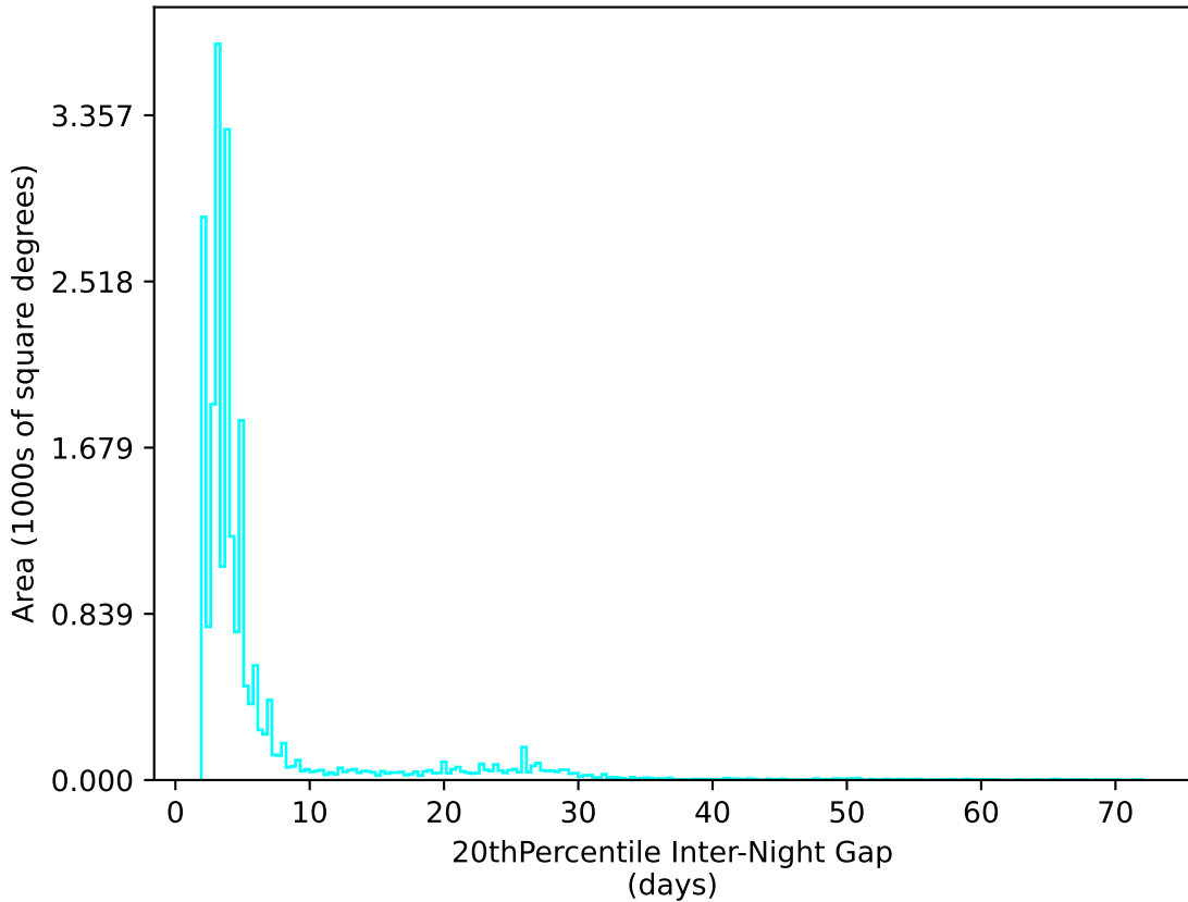
ddf_loaded_fl2_v3.4_10yrs All sky u band: 20thPercentile Inter-Night Gap
