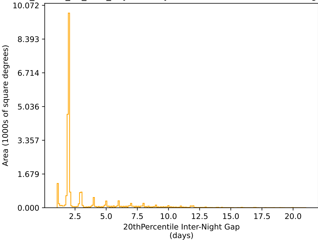
ddf_loaded_fl2_v3.4_10yrs All sky r band: 20thPercentile Inter-Night Gap
