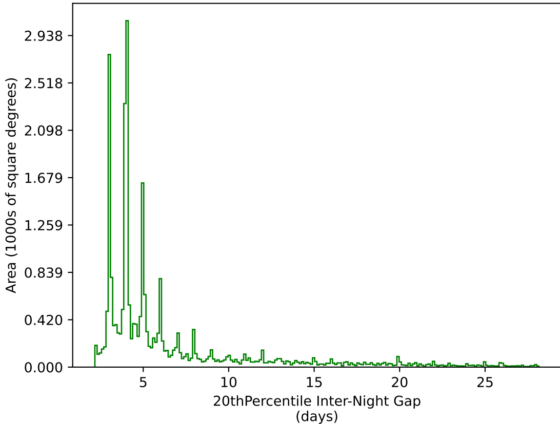
ddf_loaded_fl2_v3.4_10yrs All sky g band: 20thPercentile Inter-Night Gap
