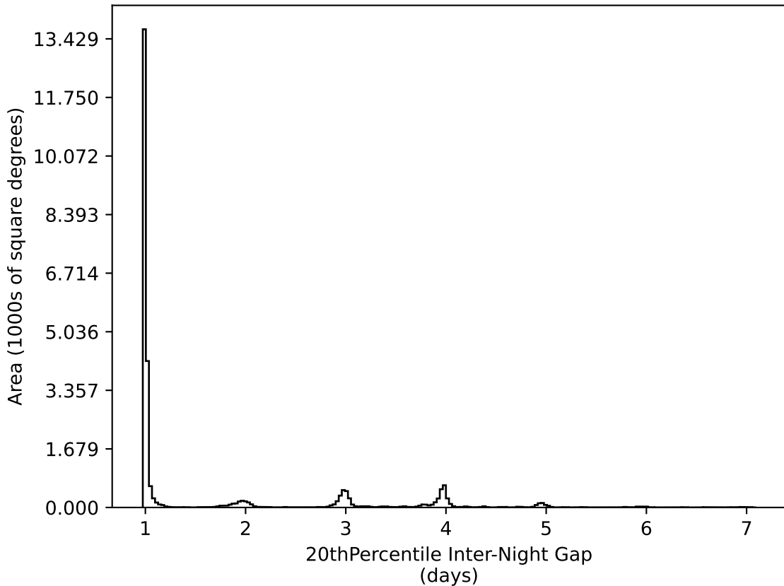
ddf_loaded_fl2_v3.4_10yrs All sky all bands: 20thPercentile Inter-Night Gap
