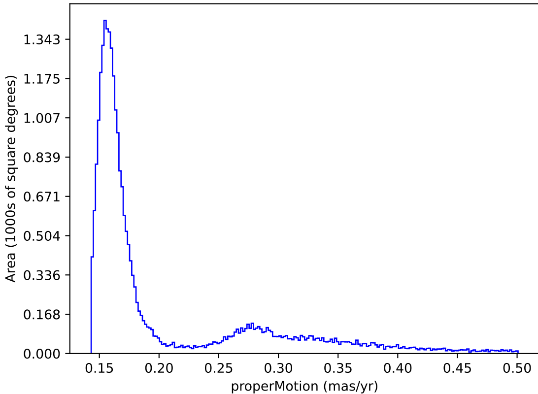
ddf_loaded_fl2_v3.4_10yrs : properMotion
