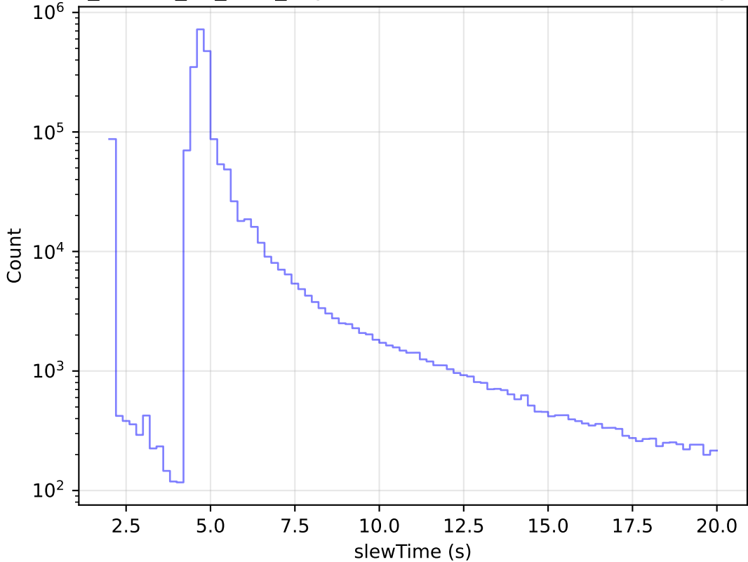
ddf_loaded_fl2_v3.4_10yrs All visits: Zoom Slew Time Histogram
