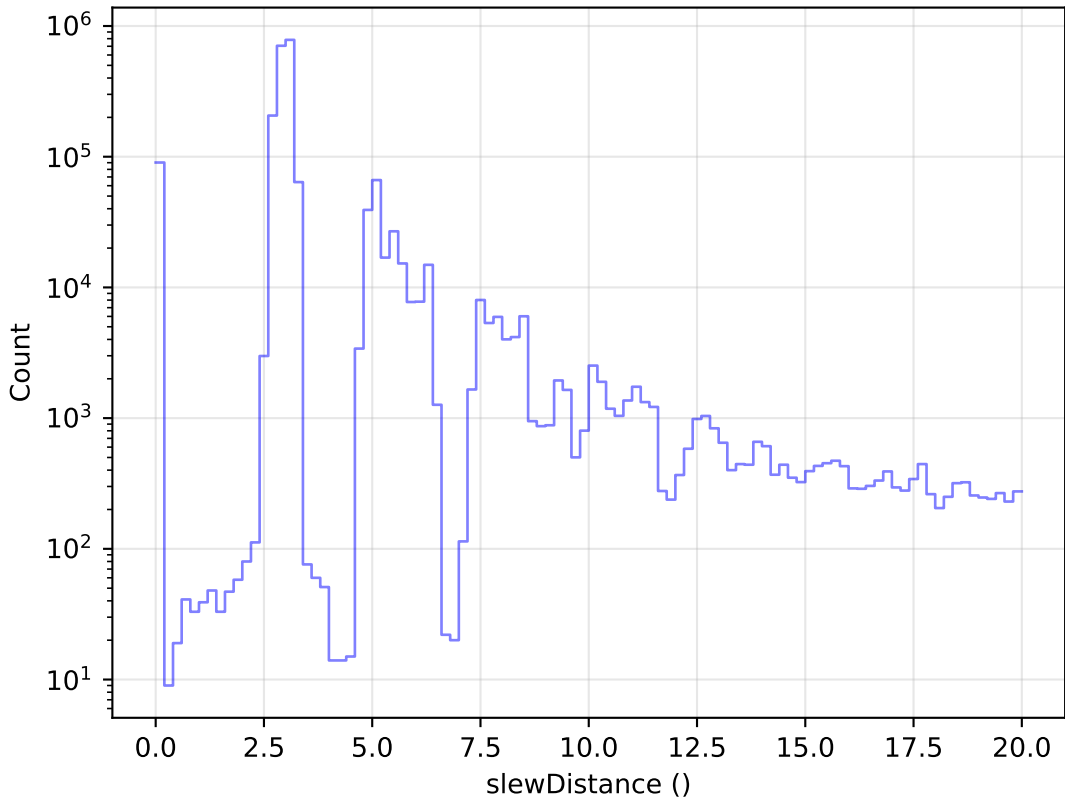
ddf_loaded_fl2_v3.4_10yrs All visits: Zoom Slew Distance Histogram
