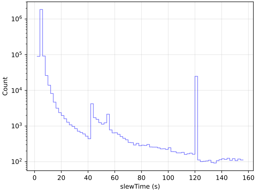
ddf_loaded_fl2_v3.4_10yrs All visits: Slew Time Histogram
