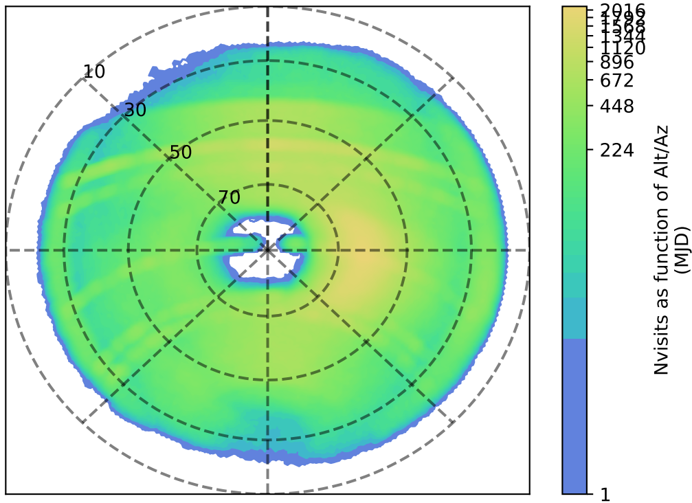
ddf_loaded_fl2_v3.4_10yrs z: Nvisits as function of Alt/Az
