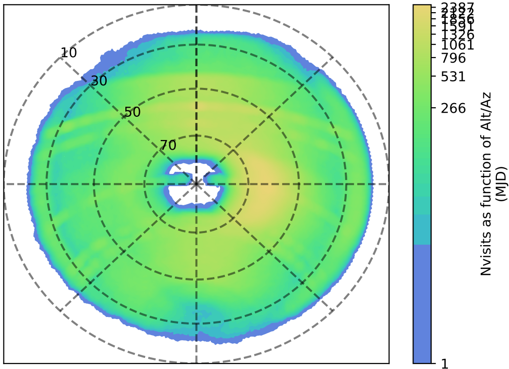
ddf_loaded_fl2_v3.4_10yrs i: Nvisits as function of Alt/Az
