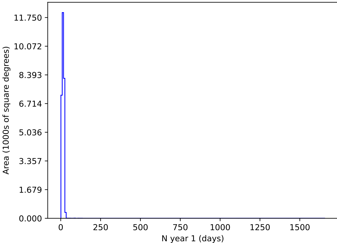
ddf_loaded_fl2_v3.4_10yrs z and night < 365: N year 1
