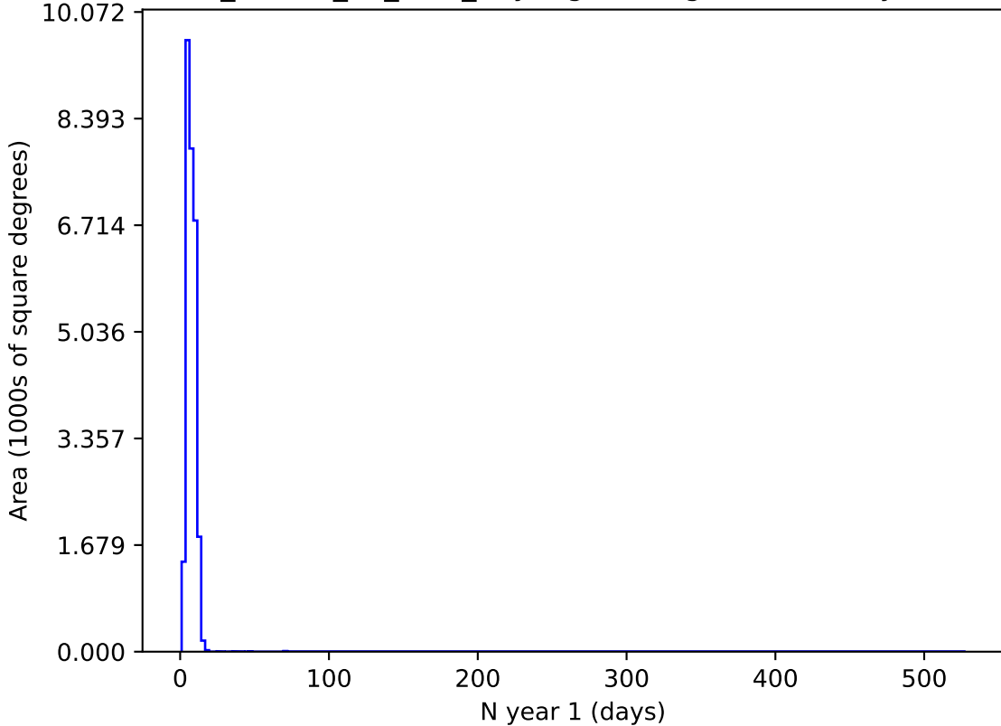
ddf_loaded_fl2_v3.4_10yrs g and night < 365: N year 1
