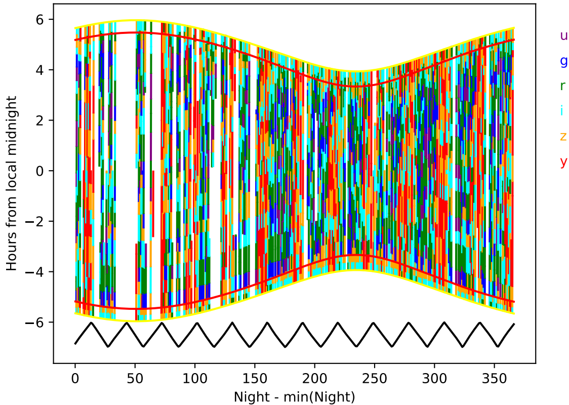
ddf_loaded_fl2_v3.4_10yrs year 8-9: Hourglass
