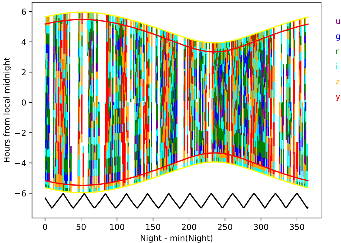
ddf_loaded_fl2_v3.4_10yrs year 7-8: Hourglass
