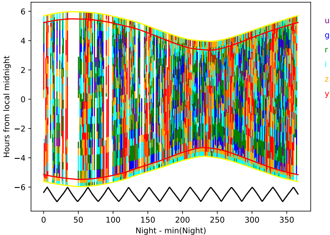
ddf_loaded_fl2_v3.4_10yrs year 6-7: Hourglass
