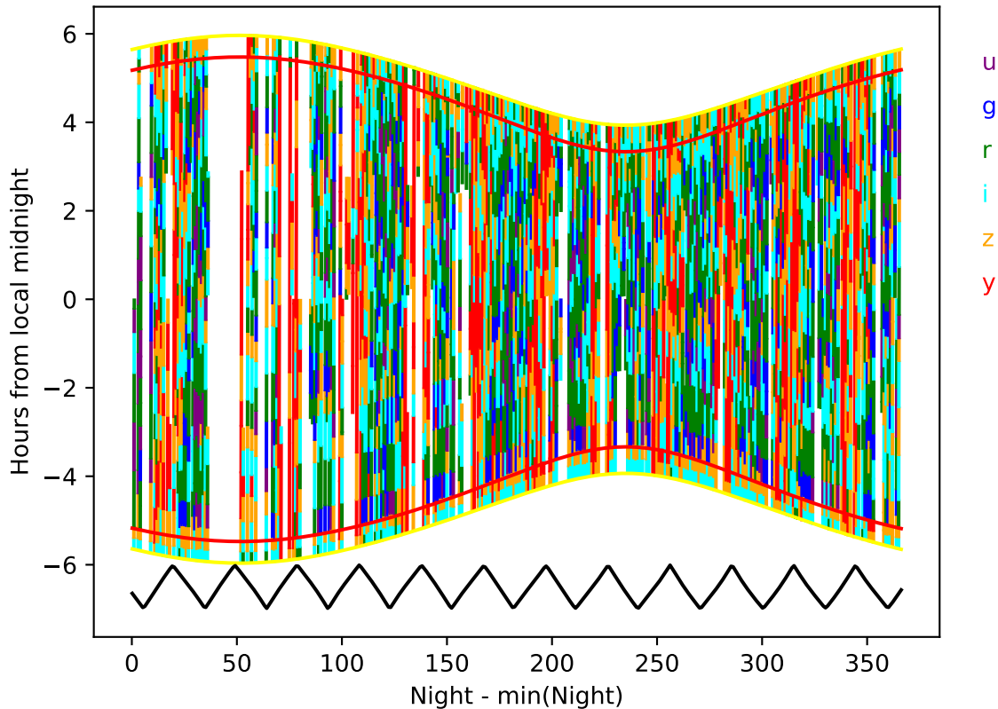
ddf_loaded_fl2_v3.4_10yrs year 2-3: Hourglass
