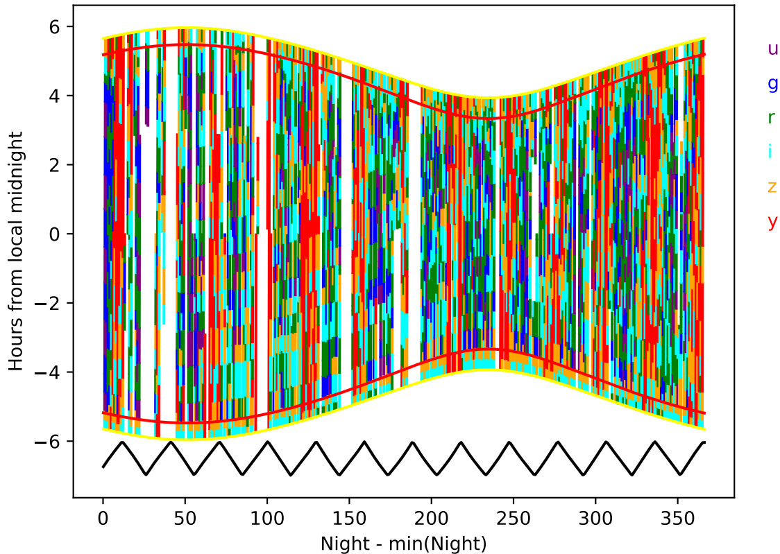
ddf_loaded_fl2_v3.4_10yrs year 0-1: Hourglass
