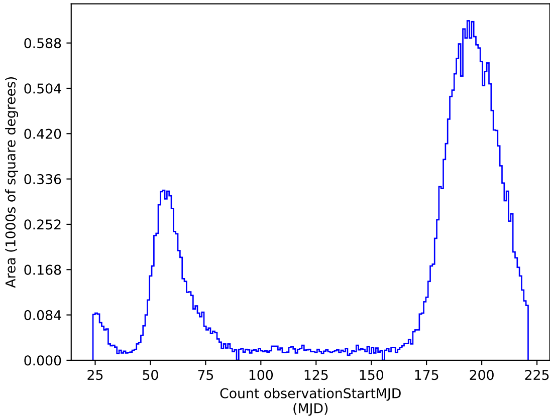
ddf_loaded_fl2_v3.4_10yrs i: Count observationStartMJD
