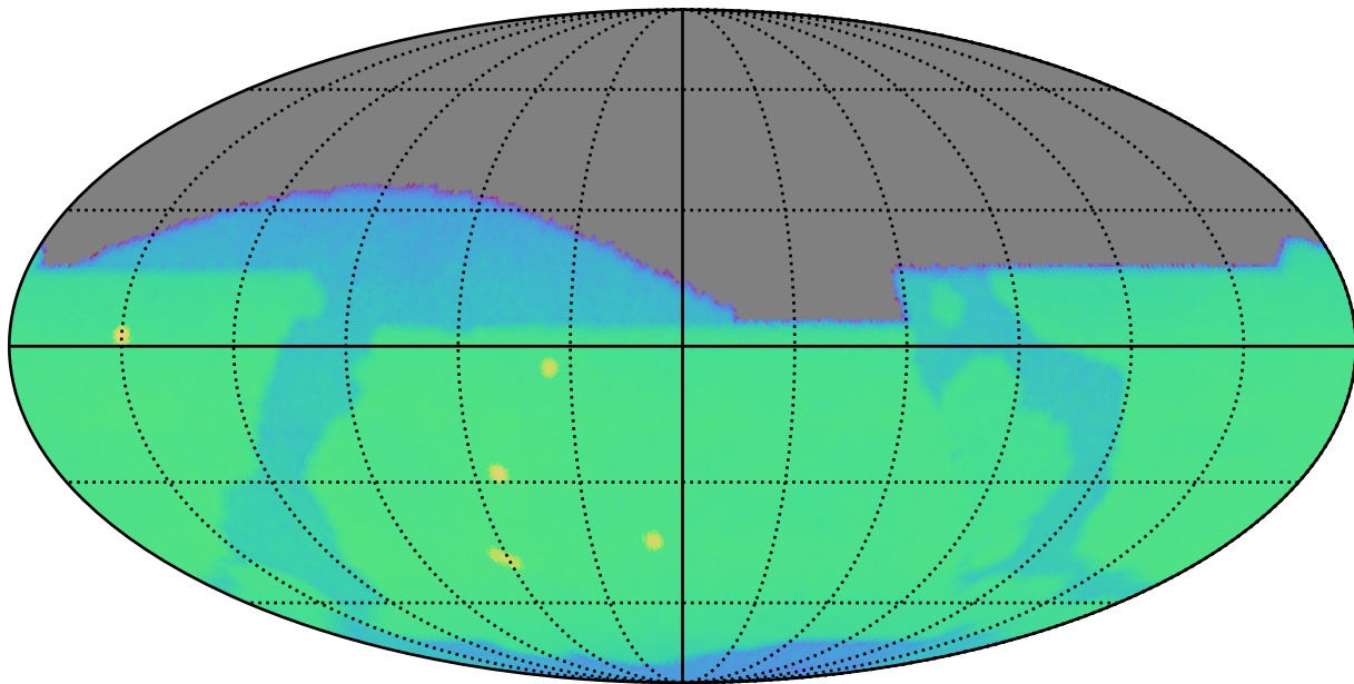
ddf_loaded_fl2_v3.4_10yrs z: CoaddM5
