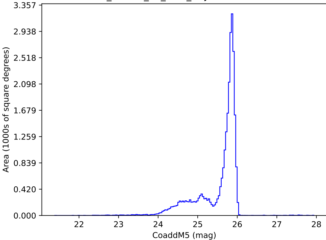
ddf_loaded_fl2_v3.4_10yrs z: CoaddM5
