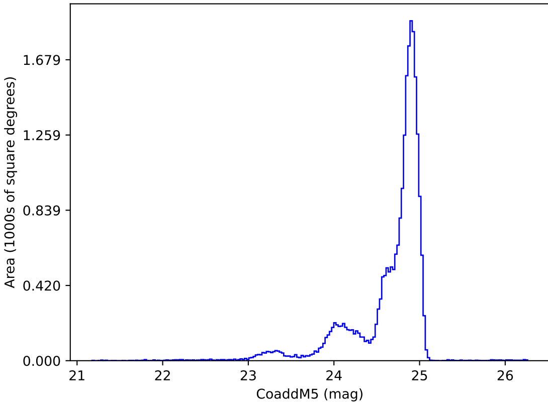
ddf_loaded_fl2_v3.4_10yrs y: CoaddM5
