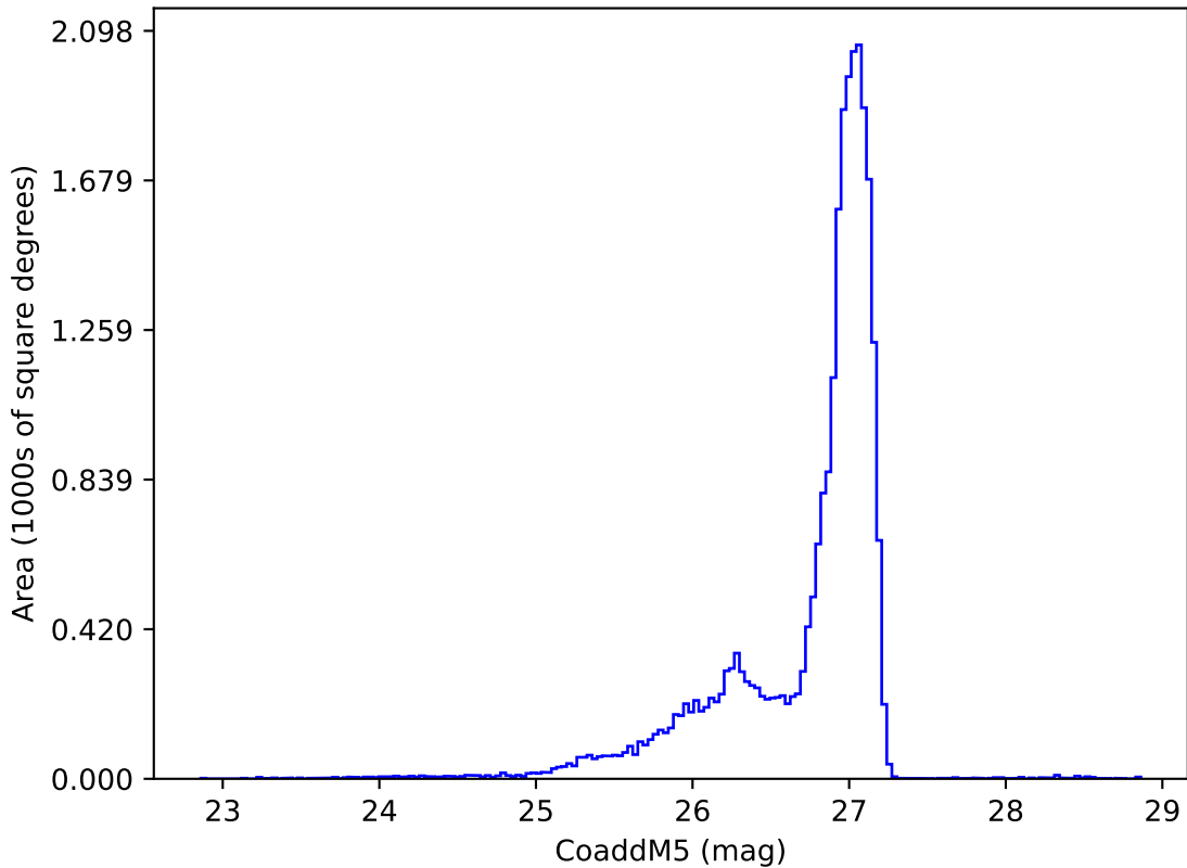
ddf_loaded_fl2_v3.4_10yrs r: CoaddM5
