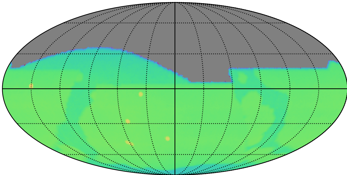
ddf_loaded_fl2_v3.4_10yrs : CoaddM5
