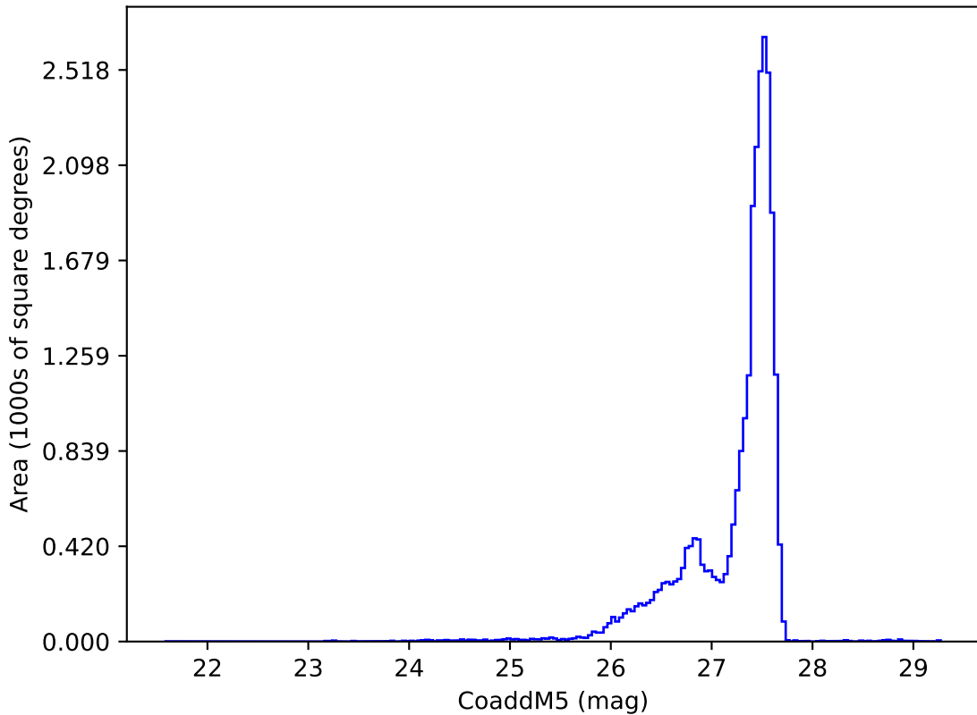
ddf_loaded_fl2_v3.4_10yrs : CoaddM5
