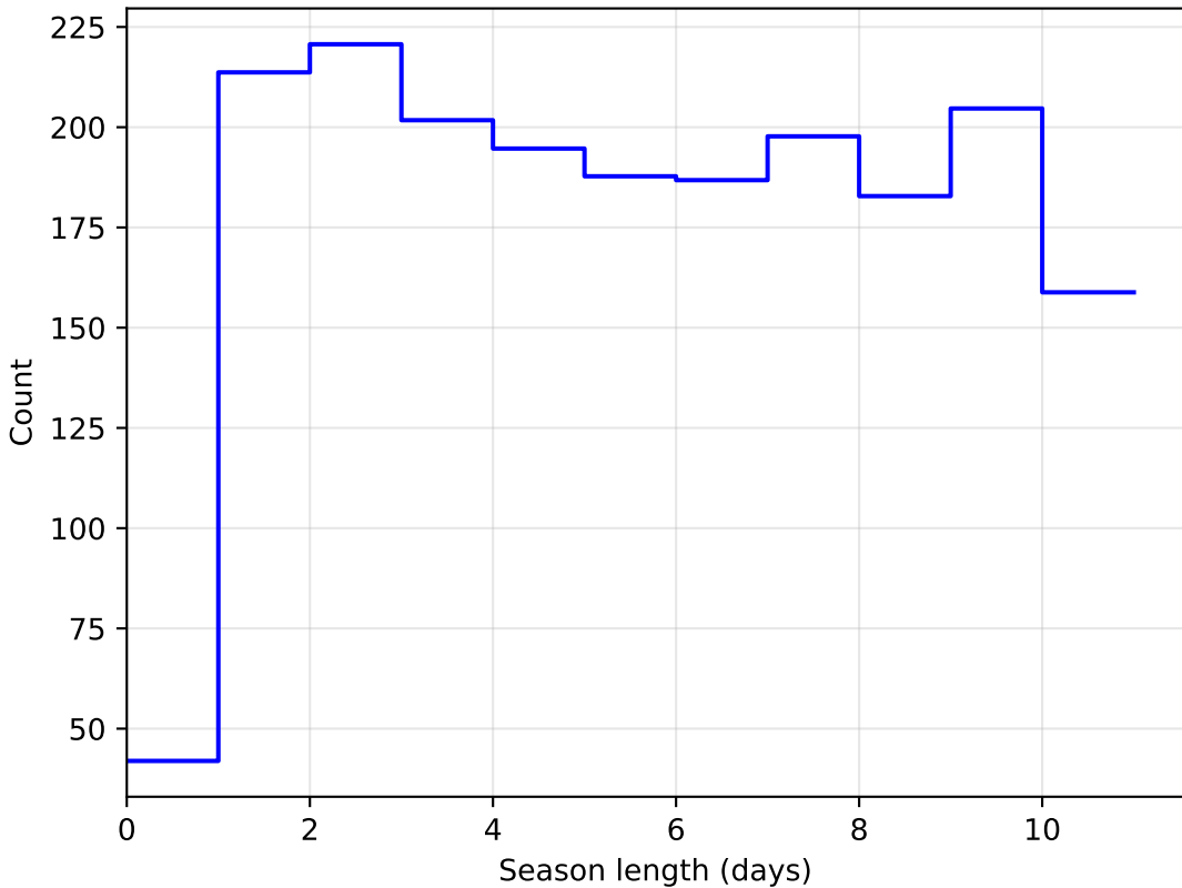
ddf_loaded_fl2_v3.4_10yrs DD: COSMOS all bands: SeasonLength
