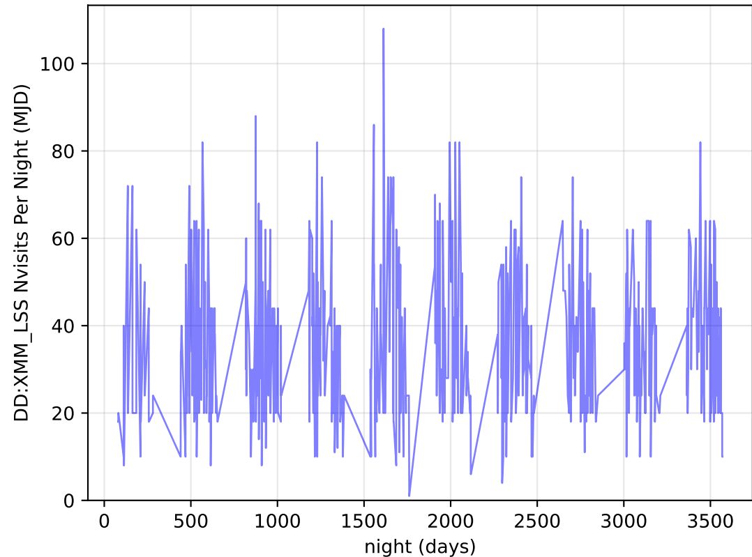
ddf_loaded_fl2_v3.4_10yrs all bands: DD:XMM_LSS Nvisits Per Night
