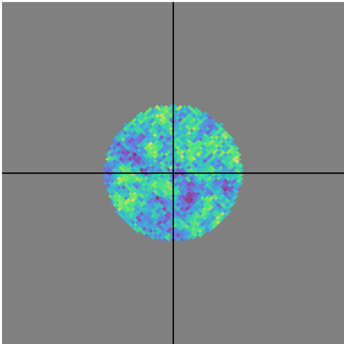
ddf_loaded_fl2_v3.4_10yrs g band: DD:WFD NVisits
