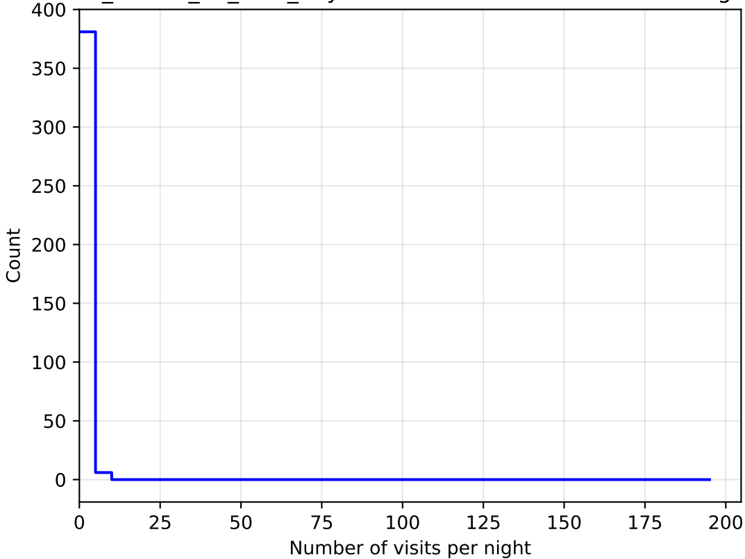
ddf_loaded_fl2_v3.4_10yrs all bands: DD:WFD NVisitsPerNight
