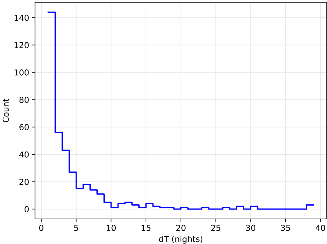
ddf_loaded_fl2_v3.4_10yrs all bands: DD:WFD Delta Nights Histogram
