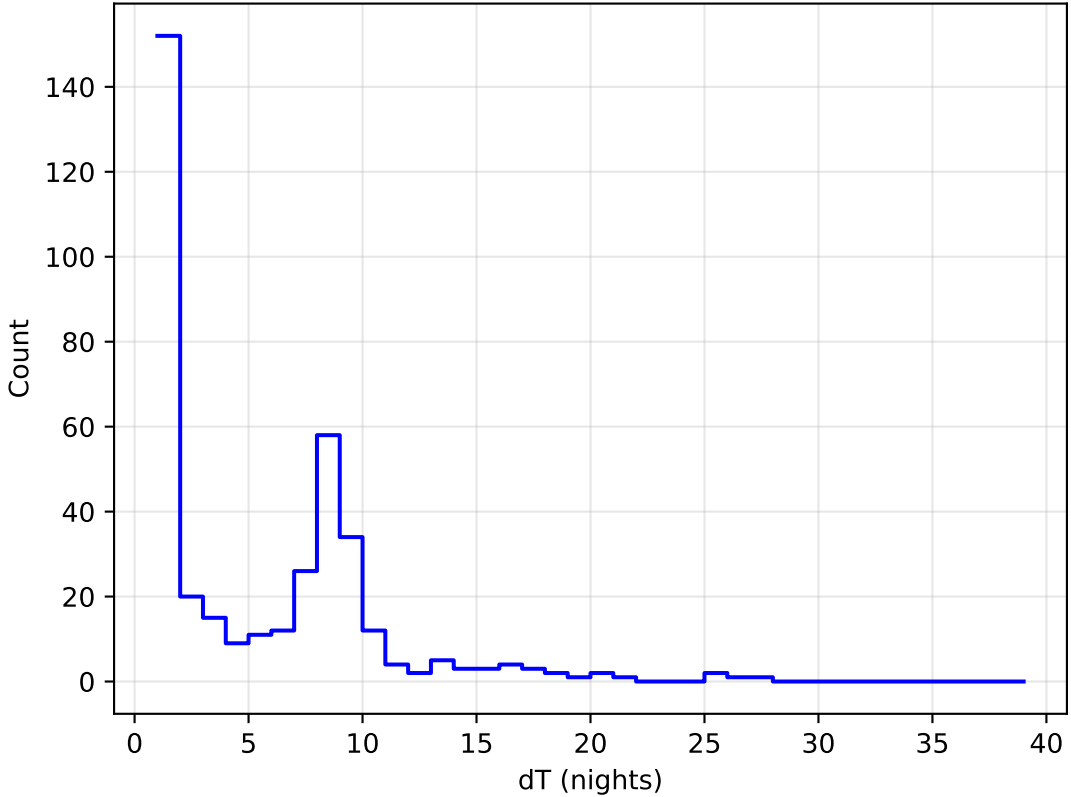
ddf_loaded_fl2_v3.4_10yrs all bands: DD:ELAISS1 Delta Nights Histogram
