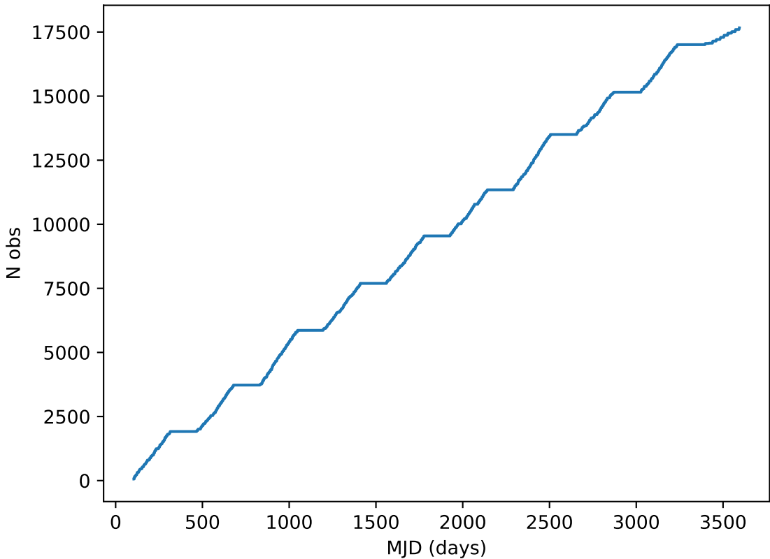
ddf_loaded_fl2_v3.4_10yrs all bands: DD:EDFS Cumulative NVisits
