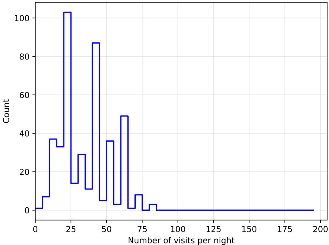
ddf_loaded_fl2_v3.4_10yrs all bands: DD:ECDFS NVisitsPerNight
