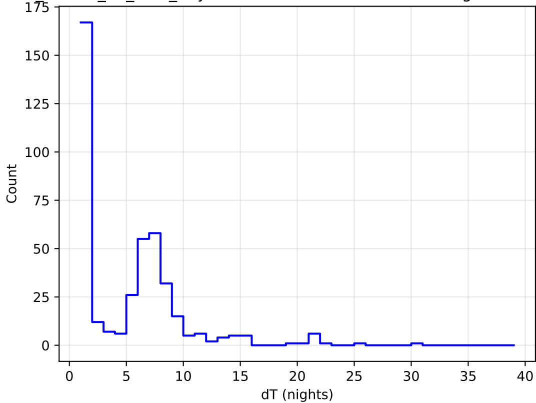
ddf_loaded_f12_v3.4_10yrs all bands: DD:ECDFS Delta Nights Histogram
