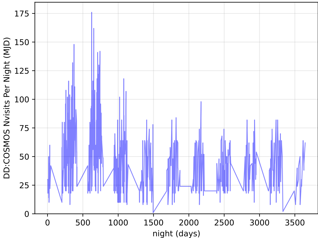
ddf_loaded_fl2_v3.4_10yrs all bands: DD: COSMOS Nvisits Per Night
