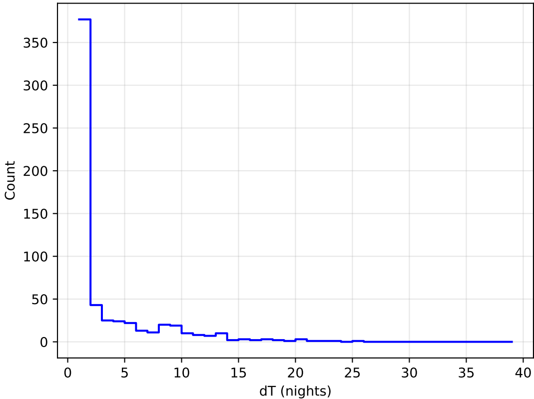
ddf_loaded_fl2_v3.4_10yrs all bands: DD: COSMOS Delta Nights Histogram
